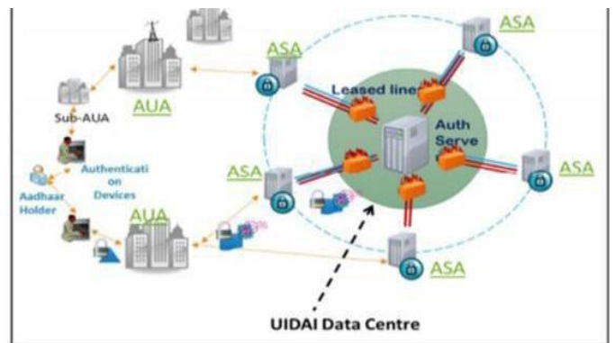
Figure.3.UDAI architecture framework
