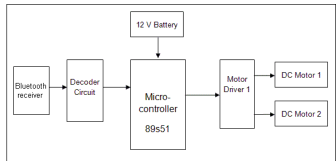
Figure.1. Block diagram of android smart phone controller Bluetooth robot using 89s51 microcontroller
