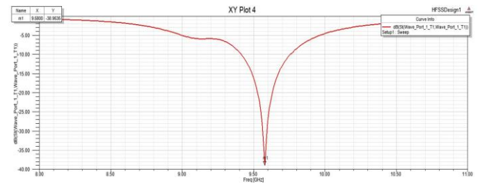
Figure. 5. (Simulated Return Loss of Antenna When Switch Is On)
