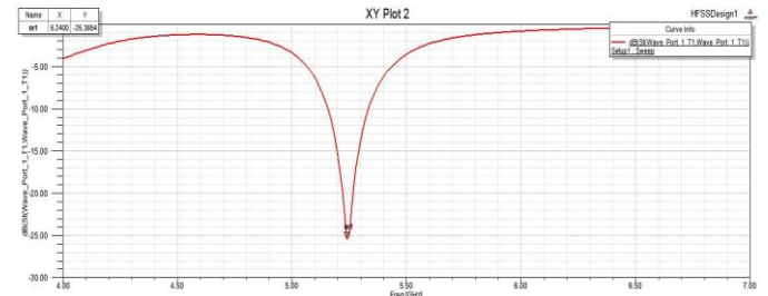
Figure.4. (simulated return loss of antenna when switch is off)
