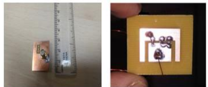
Figure.6. (fabricated antenna)
