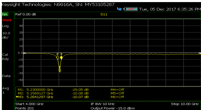
Figure.9. (measured return loss of antenna when switch is on)
