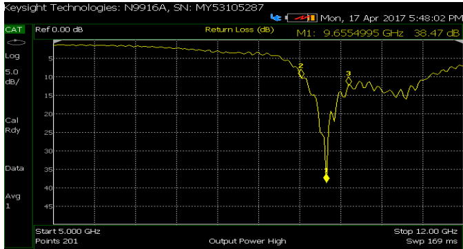
Figure.8. (measured return loss of antenna when switch is off)
