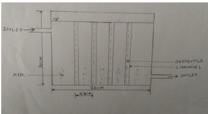
Figure.4. Cross section of GBCS (Spacing 6.5cm)
