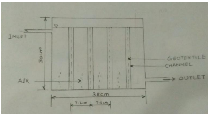
Figure.3. Cross section of GBCS (Spacing 7.6cm)
