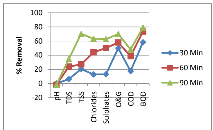
Figure.6. % Removal with change in HRT (for 4layers)
