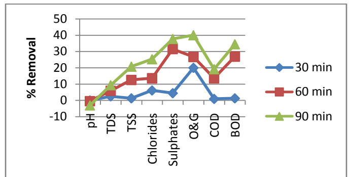
Figure.5. % Removal with change in HRT (for 2layers)
