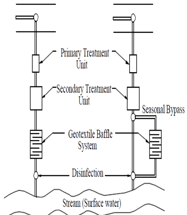
Figure.2. Installation
