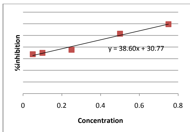
Figure. 1. DPPH radical scavenging activity of benzothiazole compound, 3d
