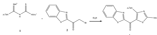
Scheme. 1. Synthetic route of molecules 3
