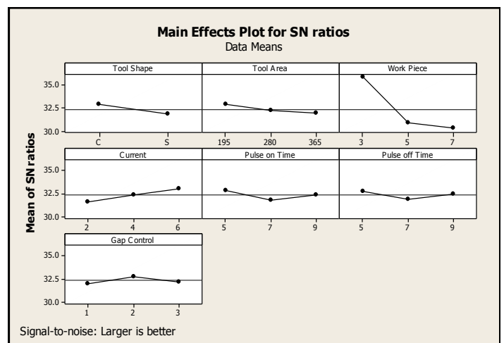
Figure. 1. Main effects plot for SN ratios for MRR
