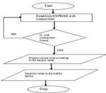
Figure.1. System Flowchart
