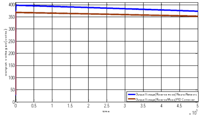
Figure.17. Comparison result of output voltage (reverse mode)
