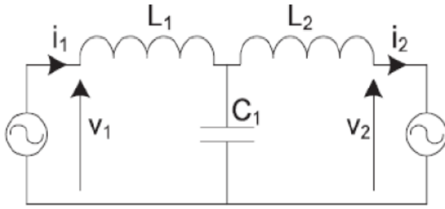
Figure.3. New Dual Active Bridge Topology
