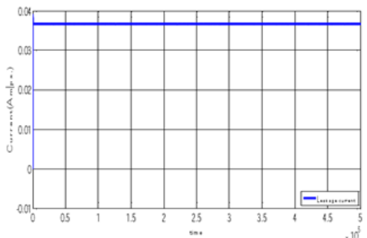
Figure.6. Leakage current level (forward mode) with PID controller
