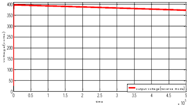
Figure.14. Battery output level voltage ANN reverse mode
