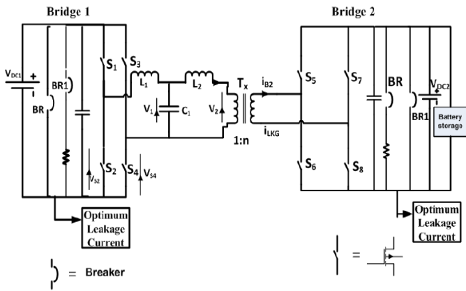
Figure.1. Proposed dual active bridge topology circuit
